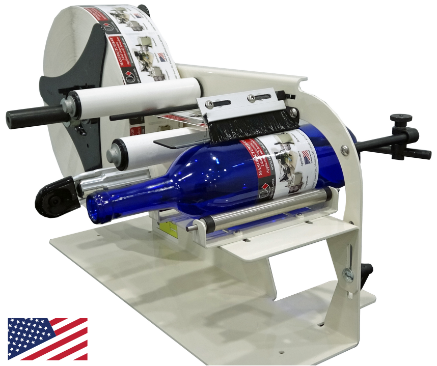
Model TAL-1100M/R Applicator
